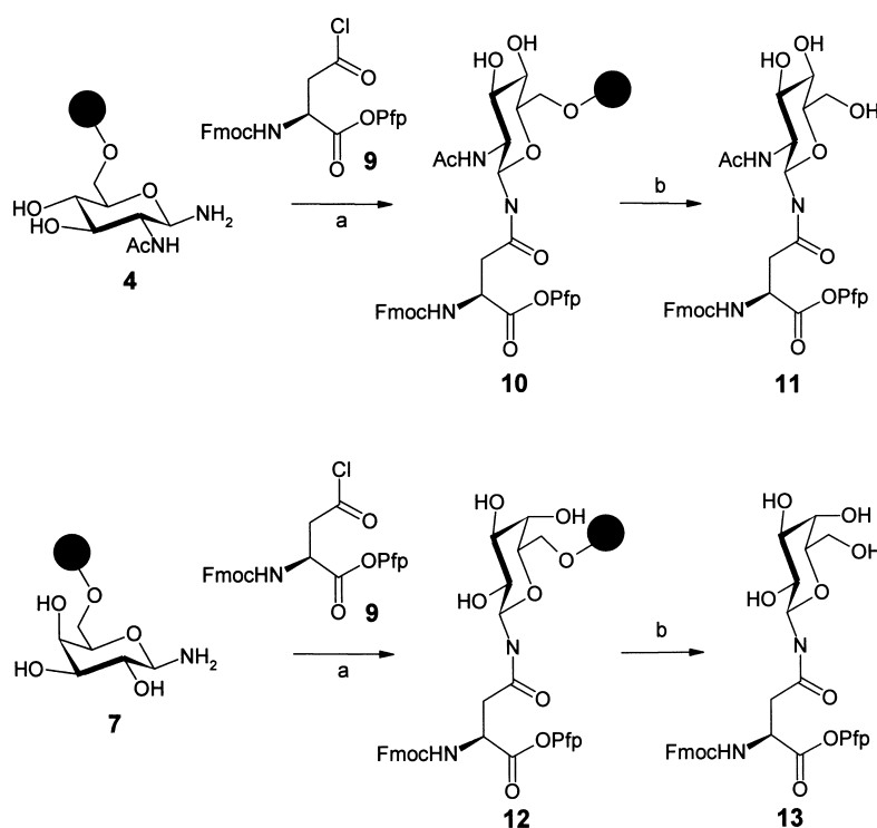
Scheme 2. Reagents and conditions: a) N -ethylmorpholine, THF, 0^\circ\text{C} –RT, 2 h; b) 2% TFA, \text{CH}_2\text{Cl}_2 , 20^\circ\text{C} , 10 min.
