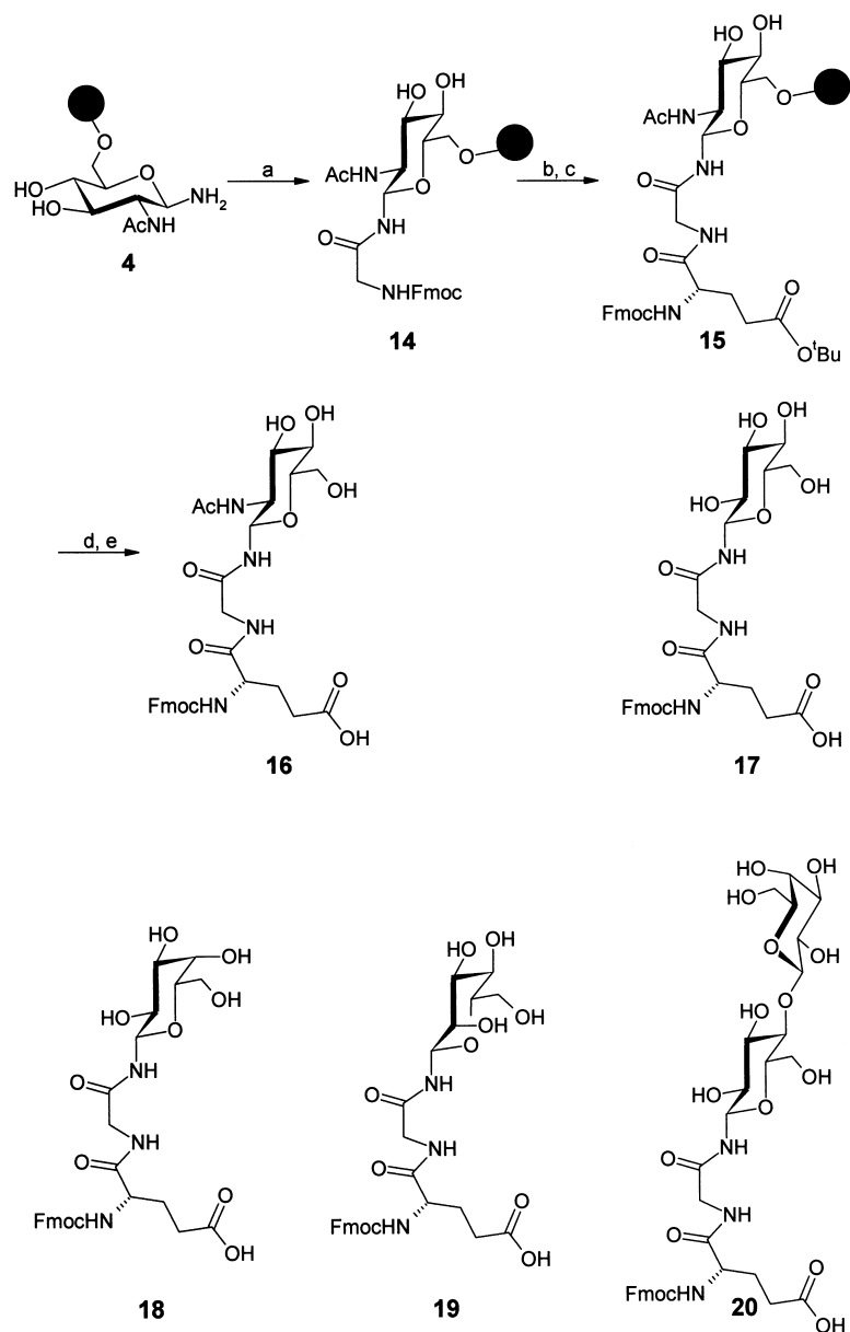
Scheme 3. Reagents and conditions: a) N α -Fmoc-Gly-OPfp, DMF, RT, 3 h; b) 20% piperidine, DMF, RT, 30 min; c) N α -Fmoc-Glu(O- t Bu)OPfp, DMF, RT, 3 h; d) 2% TFA, CH 2 Cl 2 , RT, 10 min; e) 50% TFA, CH 2 Cl 2 , RT, 30 min.
