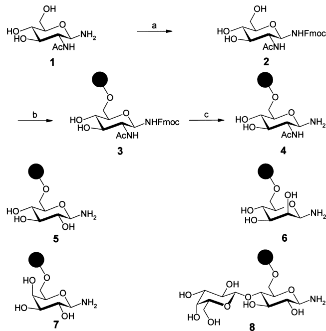
Scheme 1. Reagents and conditions: a) Fmoc-Osu, pyridine, RT, 18 h; b) trityl chloride resin, pyridine, 60^\circ\text{C} , 8 h; c) 20% piperidine, DMF, RT, 30 min. RT = room temperature.
