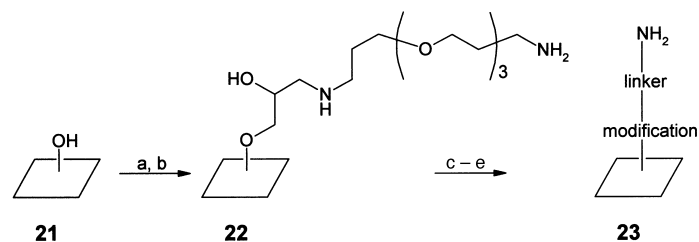
Scheme 4. Reagents and conditions: a) epibromohydrin, RT; b) 4,7,10-trioxa-1,13-tridecanediamine, RT; c) photo-labile linker (0.5 M in NMP), HATU, NMI, RT, 2 × 15 min; d) 10% Ac 2 O, 20% DIPEA, DMF, RT, 30 min; e) 20% piperidine, DMF, RT, 2 × 10 min. DIPEA = N,N' -diisopropylethylamine.
